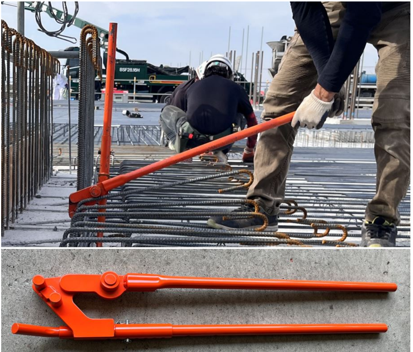
Rebar bender, max Ø12mm, adjustable
